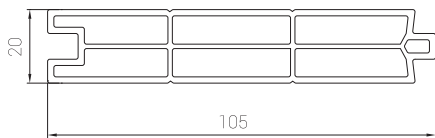
PR6022 20 mm Lambri 20 mm Panel
