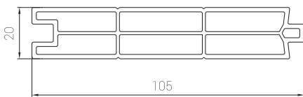
PRTS22 20 mm Lambri 20 mm Panel
