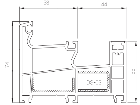
PRSY51 Dış Fix Kasa Profili Outside Fix Frame Profile
