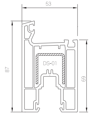
PRSY02 Kanat Profili Sash Profile
