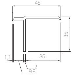
PR6031 Asimetrik T T Covering
