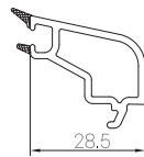
PR7117 20 mm Çıta 20 mm Glazing Bead
