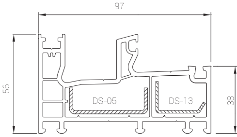
PRSY46 Fix Kasa Profili Fix Frame Profile
