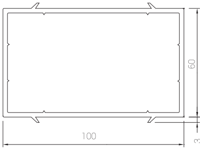
PR6034 60x100 Kutu Profili 60x100 Box Profile
