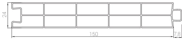
PRTS23 24 mm Lambri 24 mm Panel
