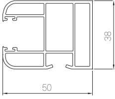
PRPJ55 Panjur Kenar Yan Ray Dikme Rail Shutter Edge Side Pillar
