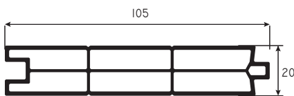
PRTS22 Lambri Panel
